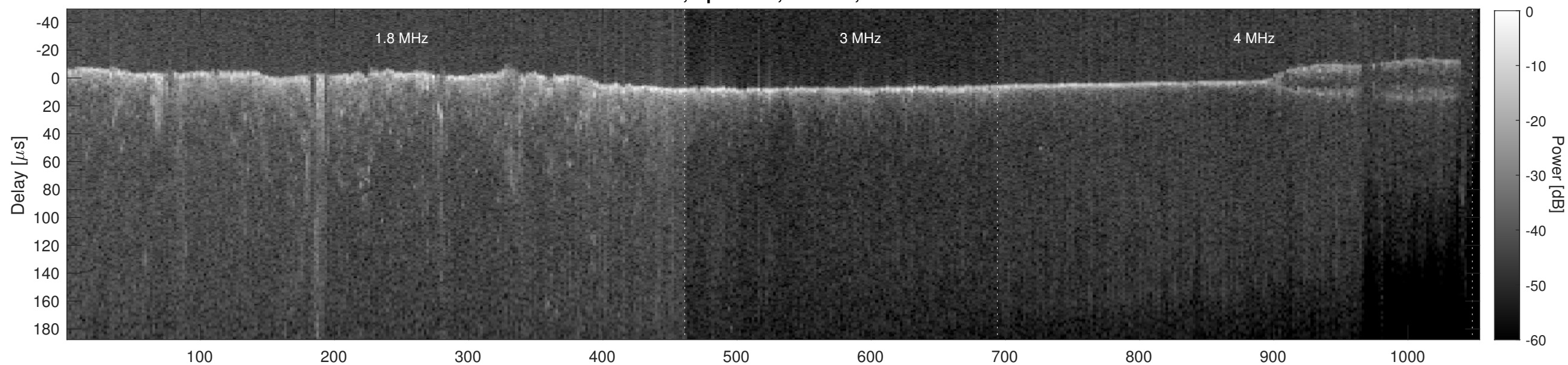
Orbit 7969, Cluttergram
