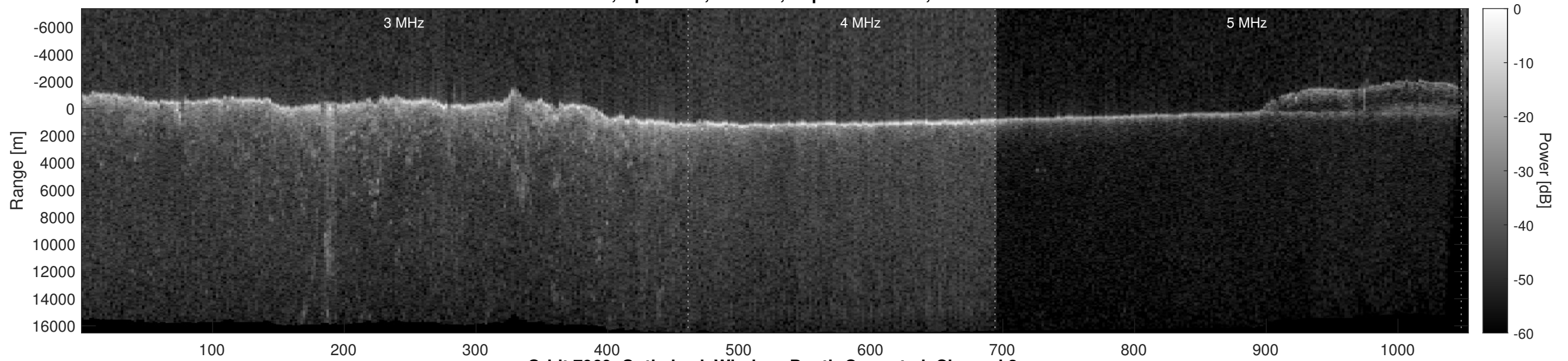
Orbit 7969, Optimized, Window, Depth-Corrected, Channel 2
