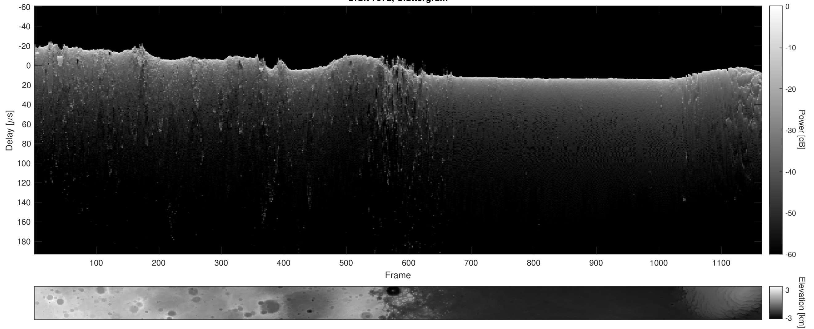
Orbit 7972, Cluttergram
