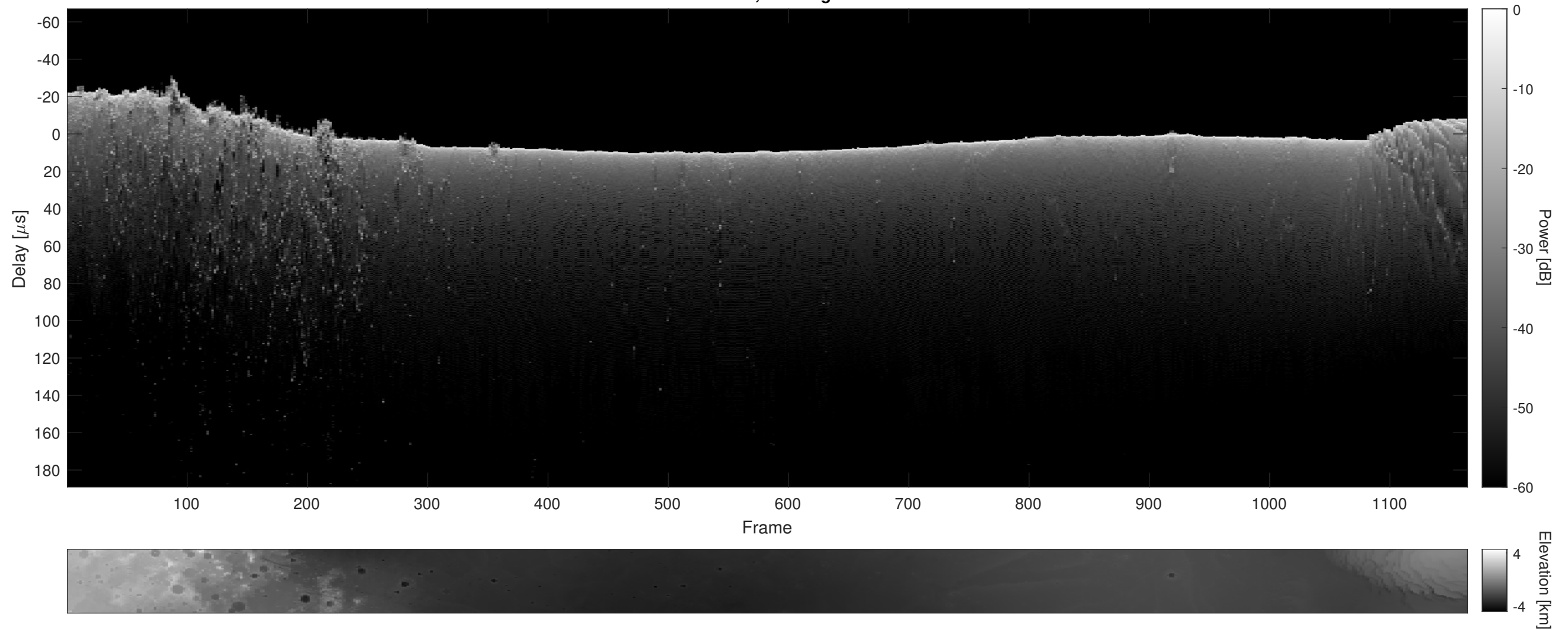
Orbit 7975, Cluttergram
