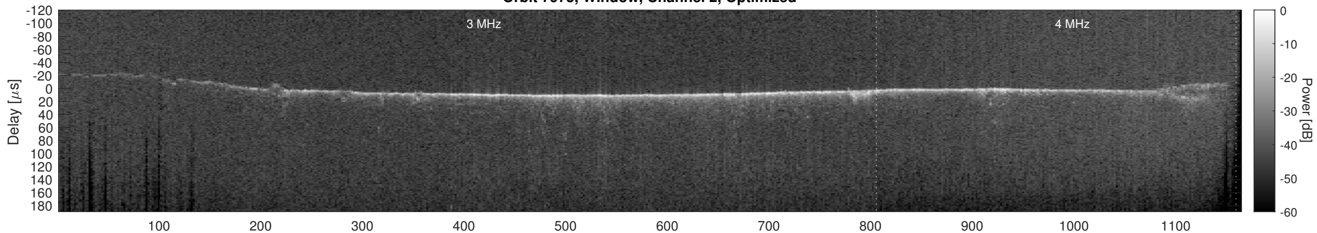
Orbit 7975, Cluttergram
