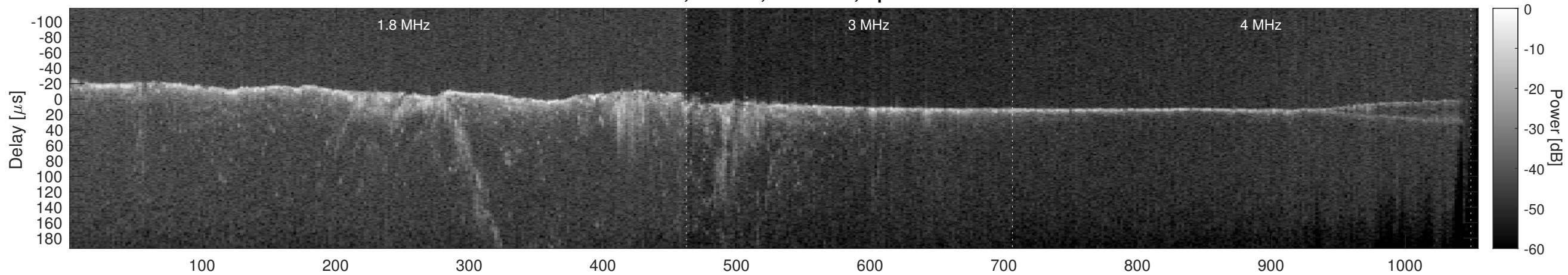
Orbit 7979, Cluttergram
