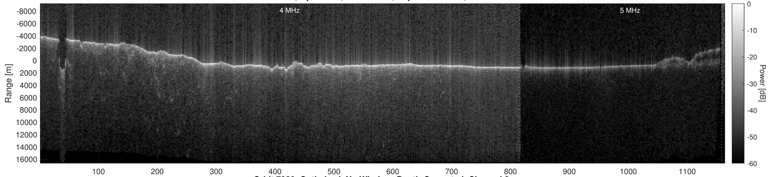
Orbit 7980, Optimized, No Window, Depth-Corrected, Channel 2
