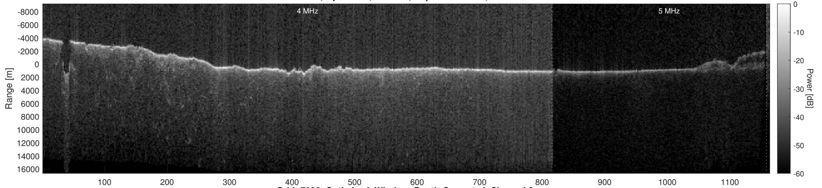
Orbit 7980, Optimized, Window, Depth-Corrected, Channel 2
