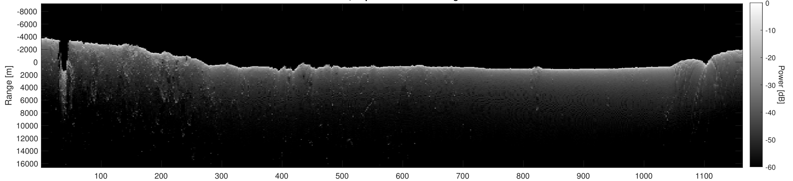
Orbit 7980, Depth-Corrected Cluttergram
