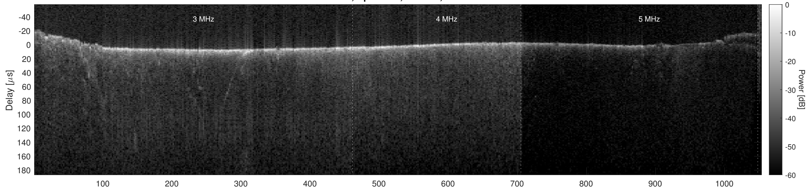
Orbit 7981, Optimized, Window, Channel 2
