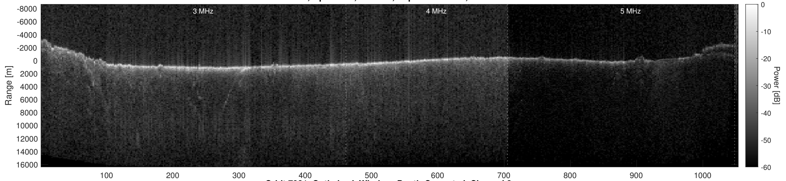
Orbit 7981, Optimized, Window, Depth-Corrected, Channel 2
