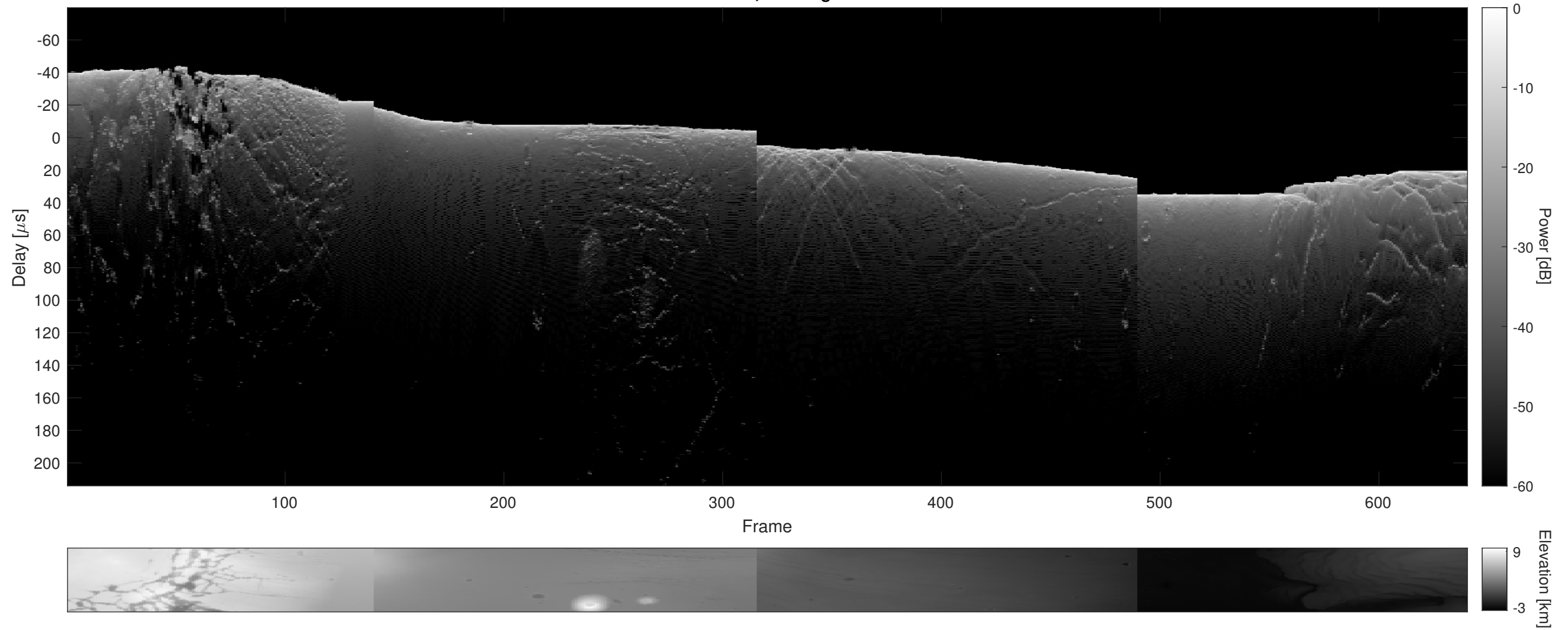
Orbit 7984, Cluttergram
