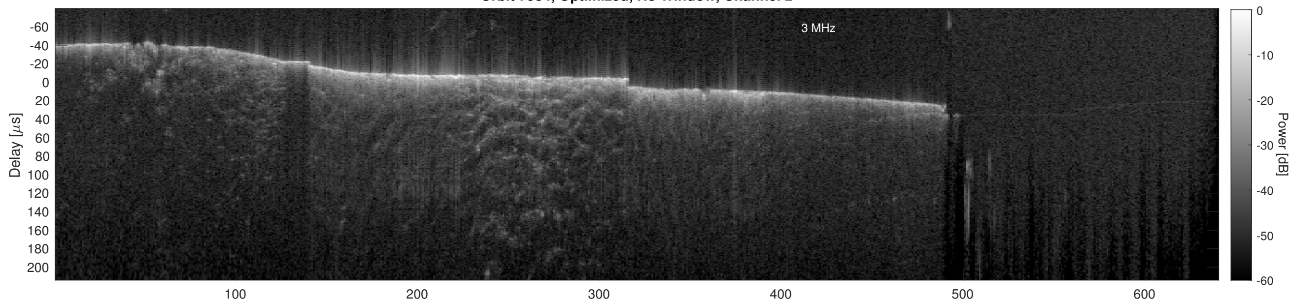
Orbit 7984, Cluttergram
