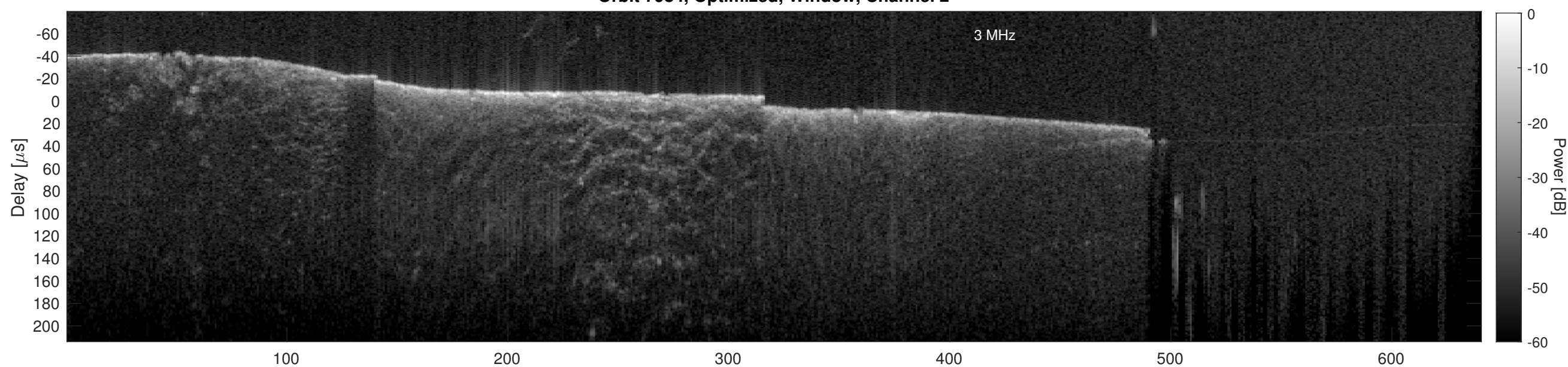
Orbit 7984, Cluttergram
