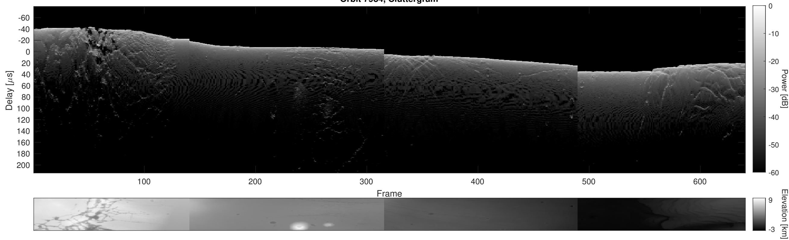
Orbit 7984, Cluttergram
