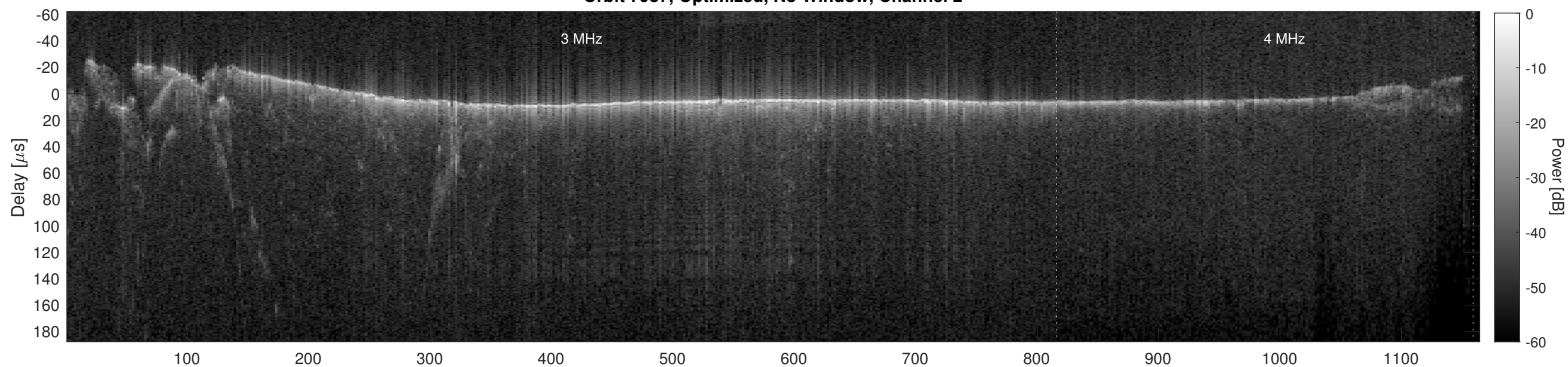
Orbit 7987, Cluttergram
