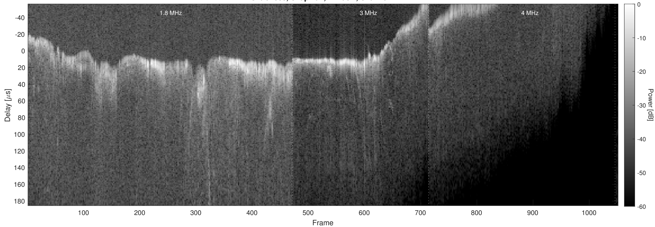
Orbit 7988, Chapman, Window, Channel 2
