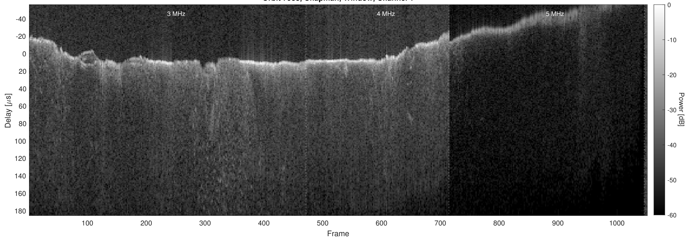
Orbit 7988, Chapman, Window, Channel 2
