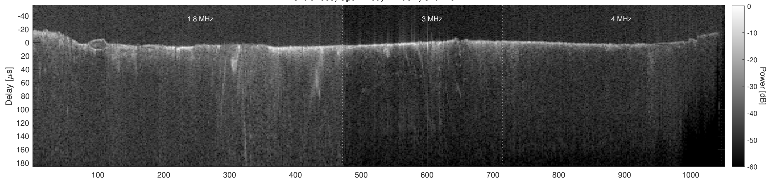
Orbit 7988, Cluttergram
