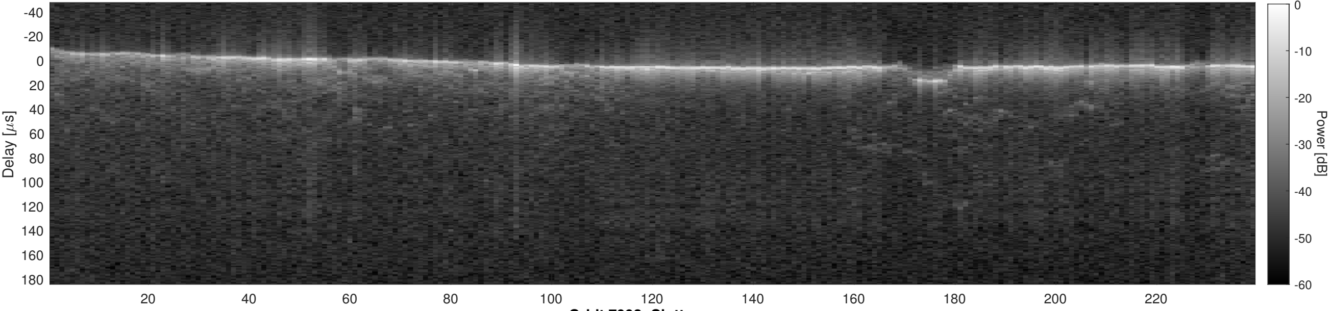
Orbit 7992, Cluttergram
