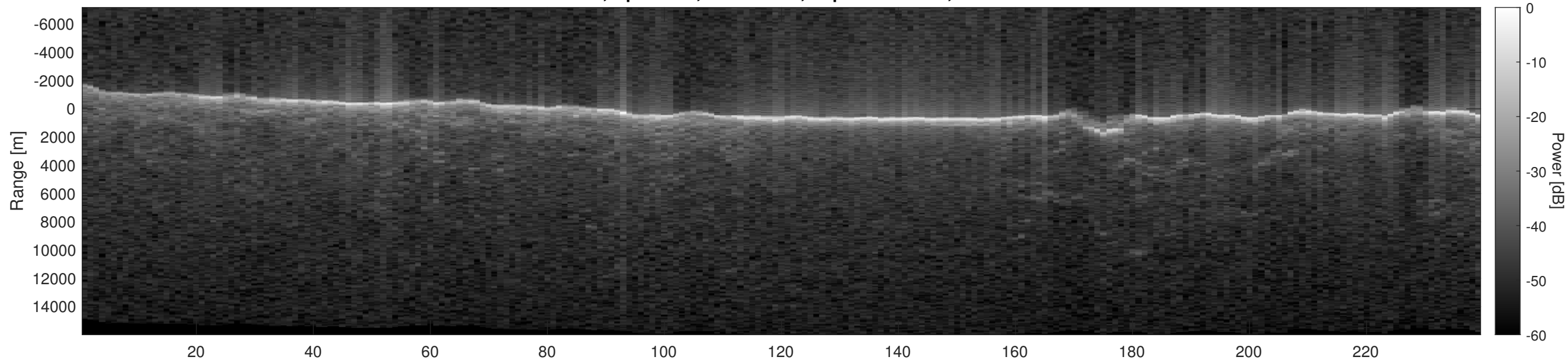
Orbit 7992, Optimized, No Window, Depth-Corrected, Channel 2
