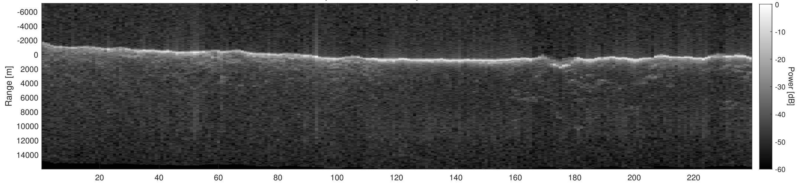
Orbit 7992, Depth-Corrected Cluttergram
