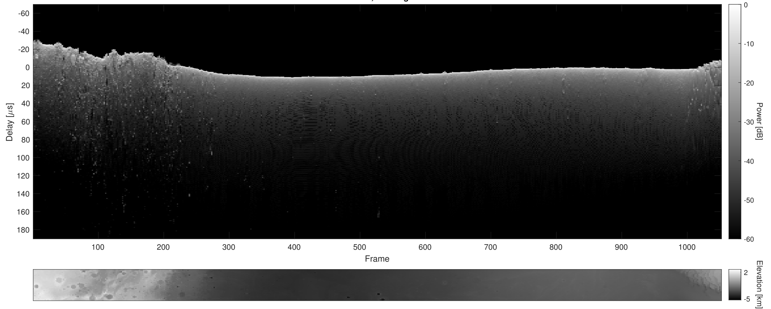
Orbit 7996, Cluttergram
