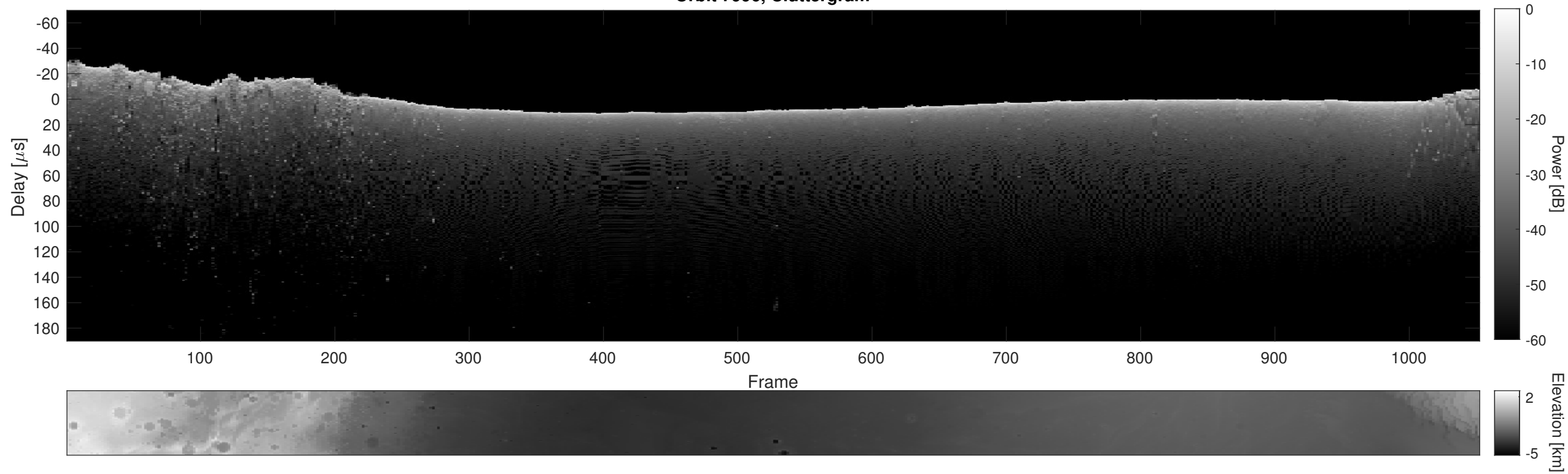
Orbit 7996, Cluttergram
