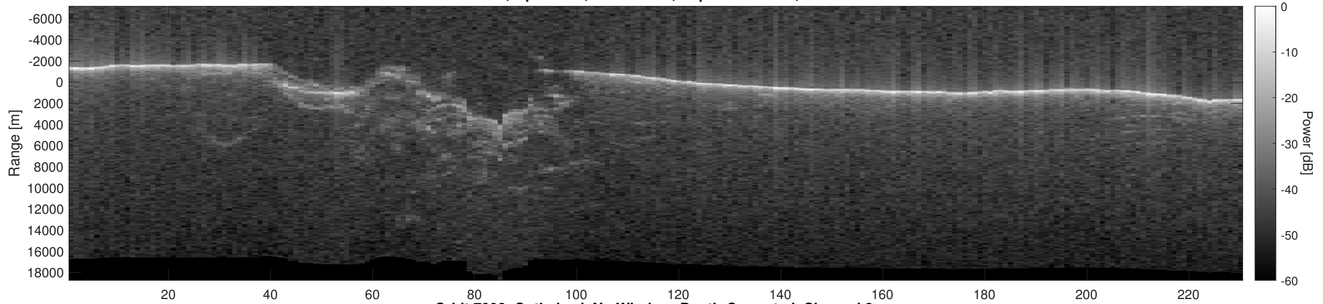
Orbit 7998, Optimized, No Window, Depth-Corrected, Channel 2
