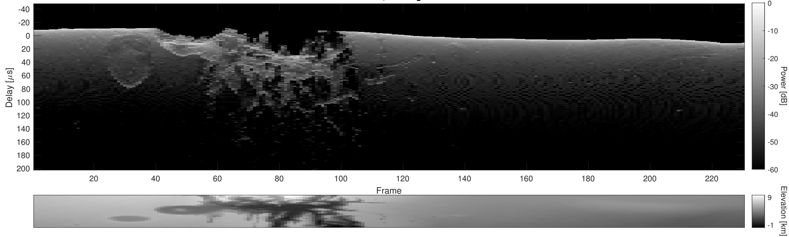
Orbit 7998, Cluttergram
