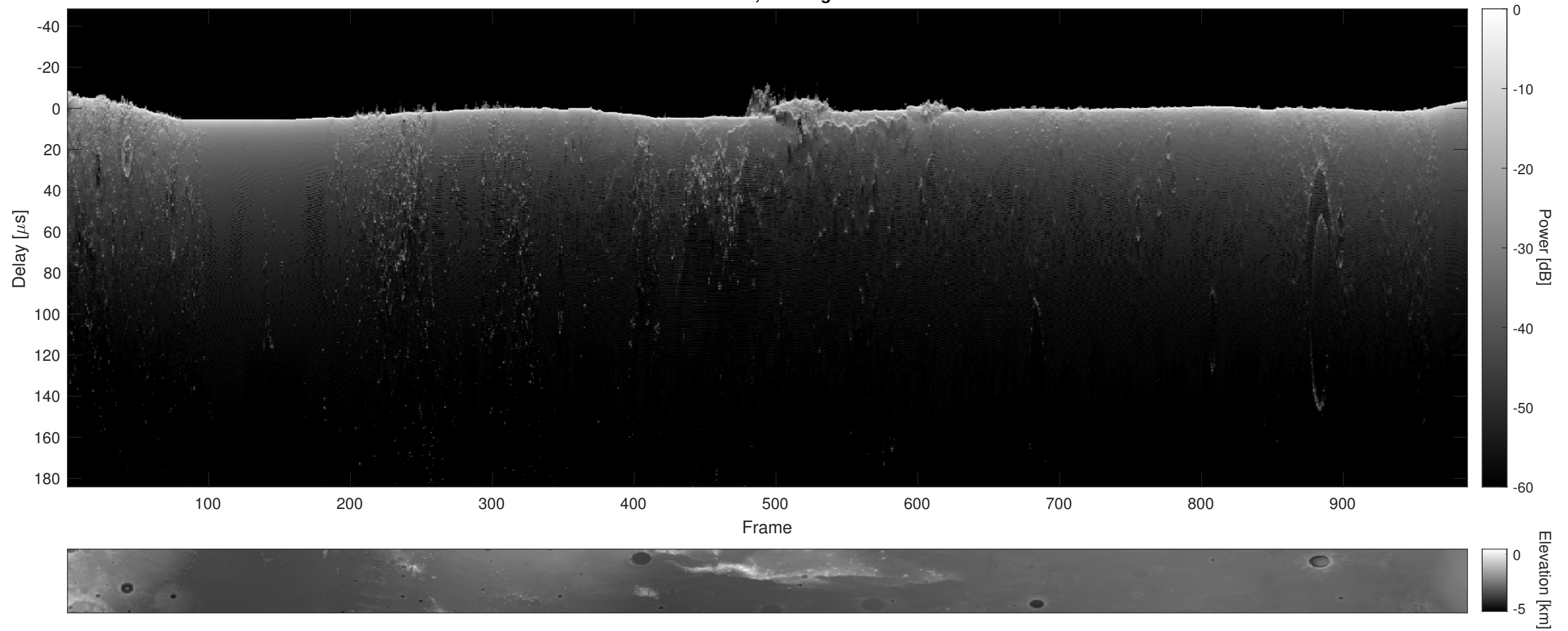
Orbit 7999, Cluttergram
