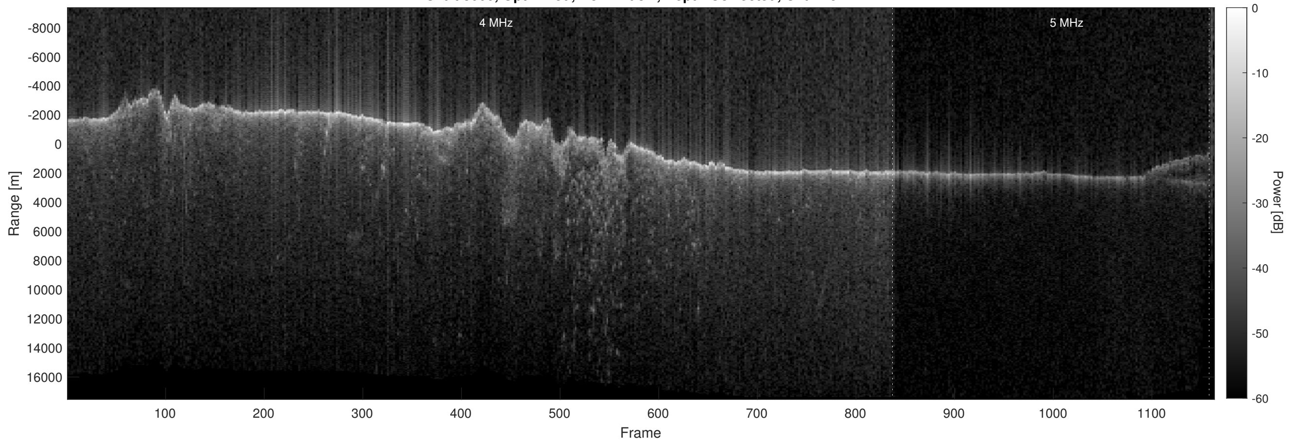
Orbit 8000, Optimized, No Window, Depth-Corrected, Channel 2
