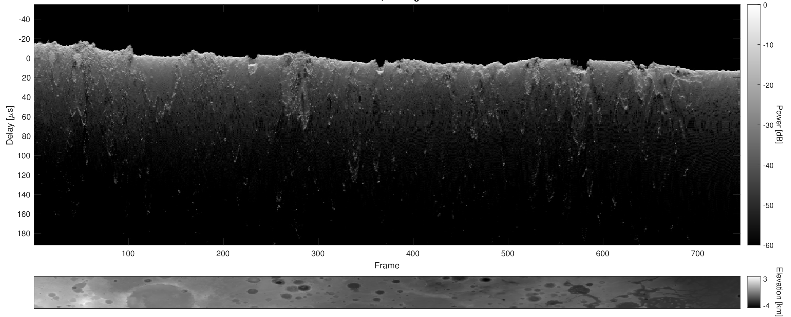
Orbit 8004, Cluttergram
