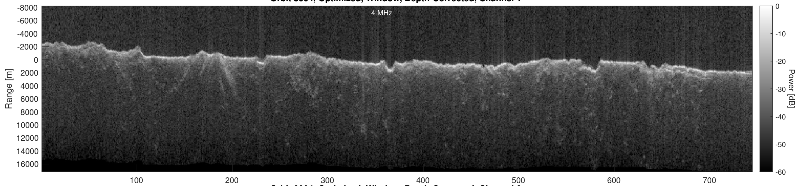
Orbit 8004, Optimized, Window, Depth-Corrected, Channel 2
