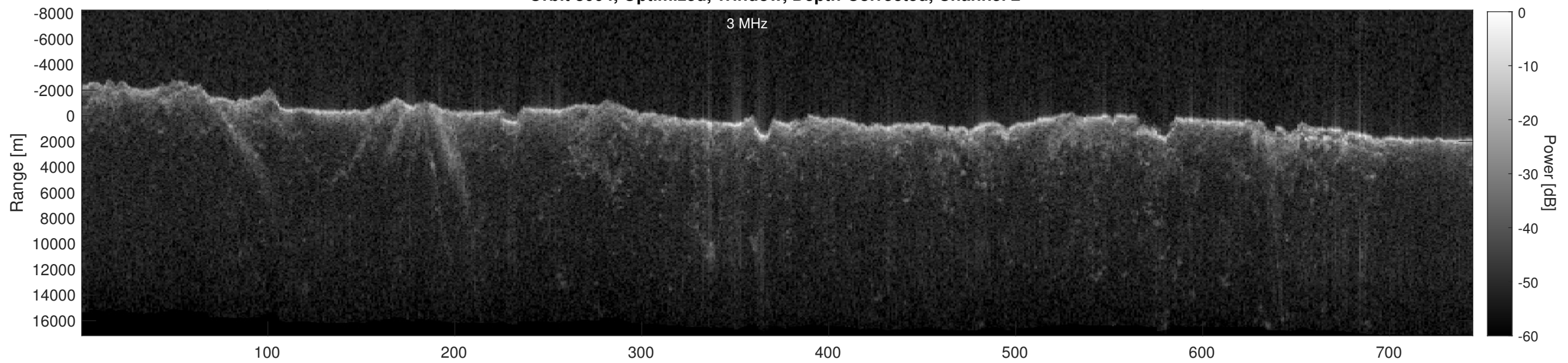
Orbit 8004, Depth-Corrected Cluttergram
