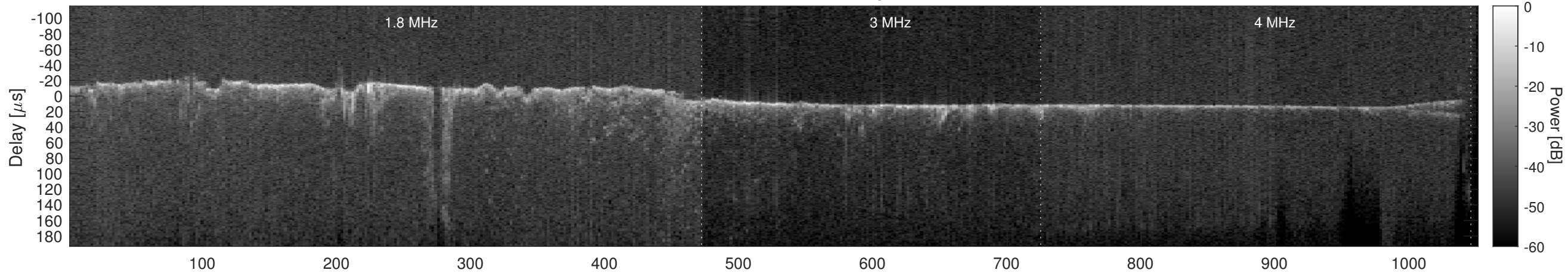
Orbit 8007, Cluttergram
