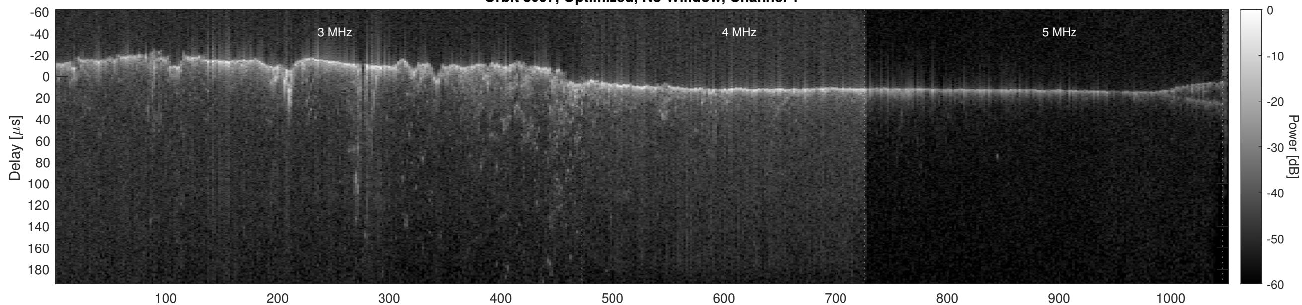
Orbit 8007, Optimized, No Window, Channel 2
