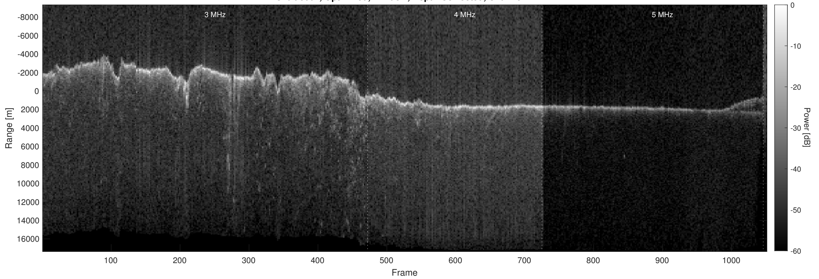
Orbit 8007, Optimized, Window, Depth-Corrected, Channel 2
