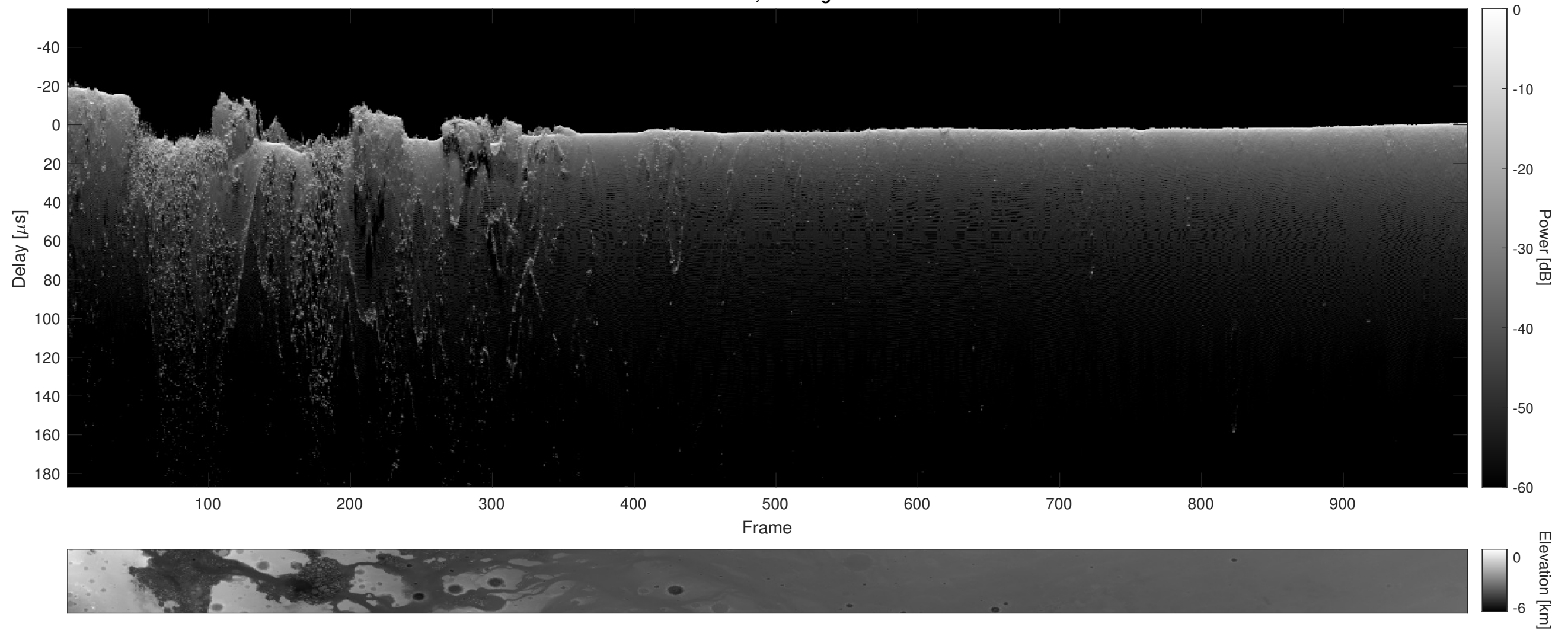
Orbit 8008, Cluttergram
