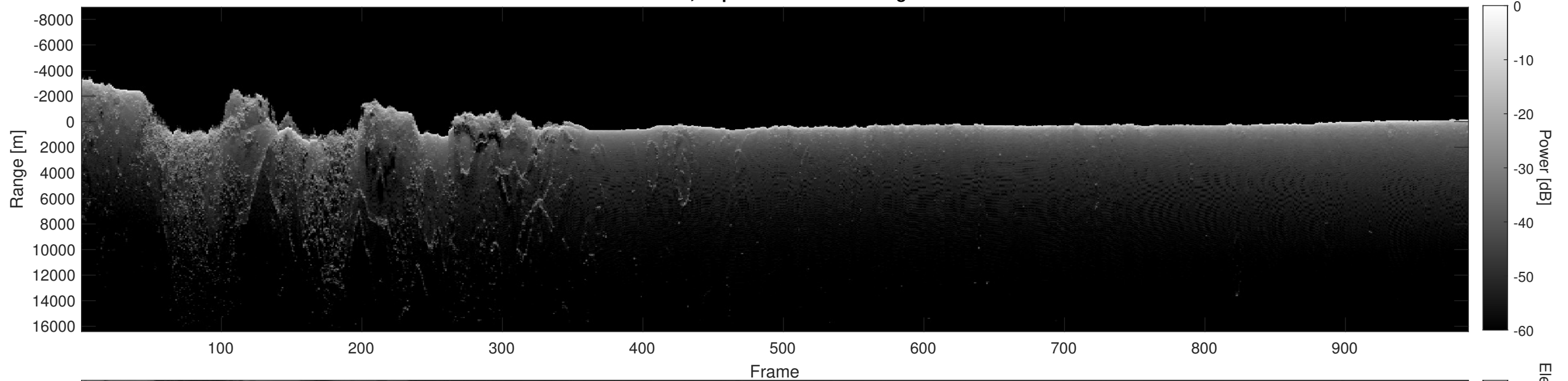
Orbit 8008, Depth-Corrected Cluttergram
