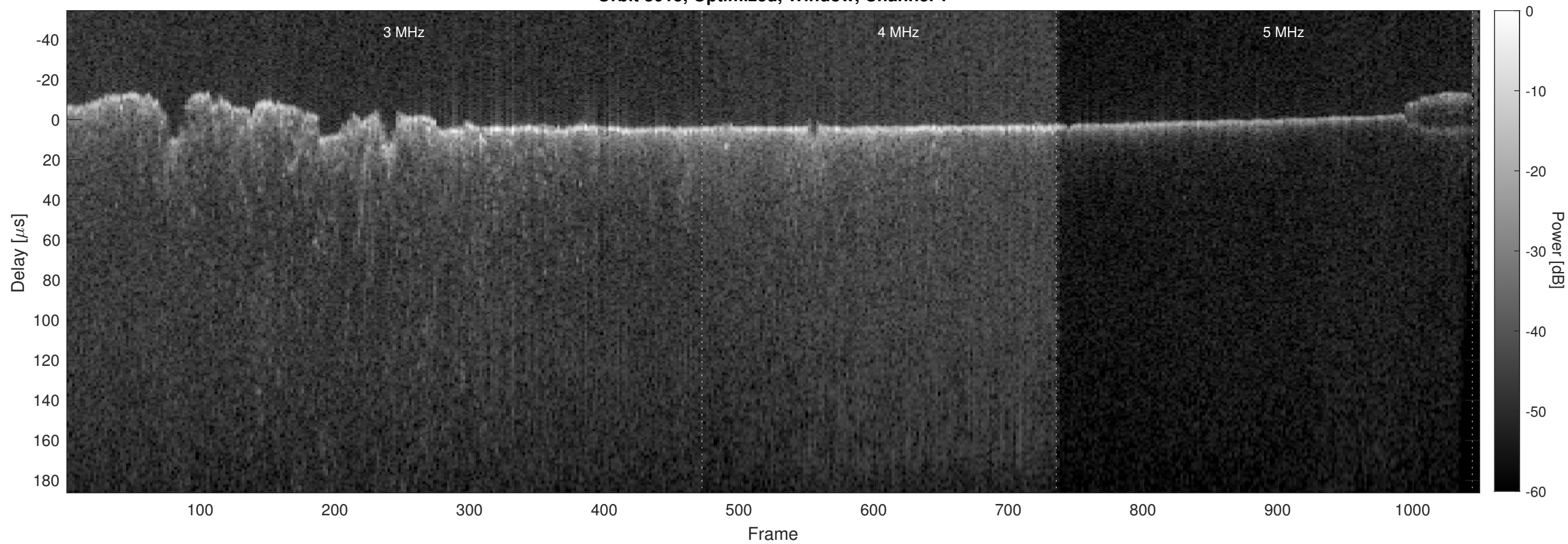
Orbit 8015, Optimized, Window, Channel 2
