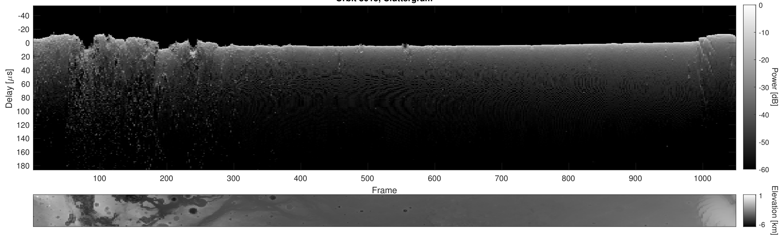
Orbit 8015, Cluttergram
