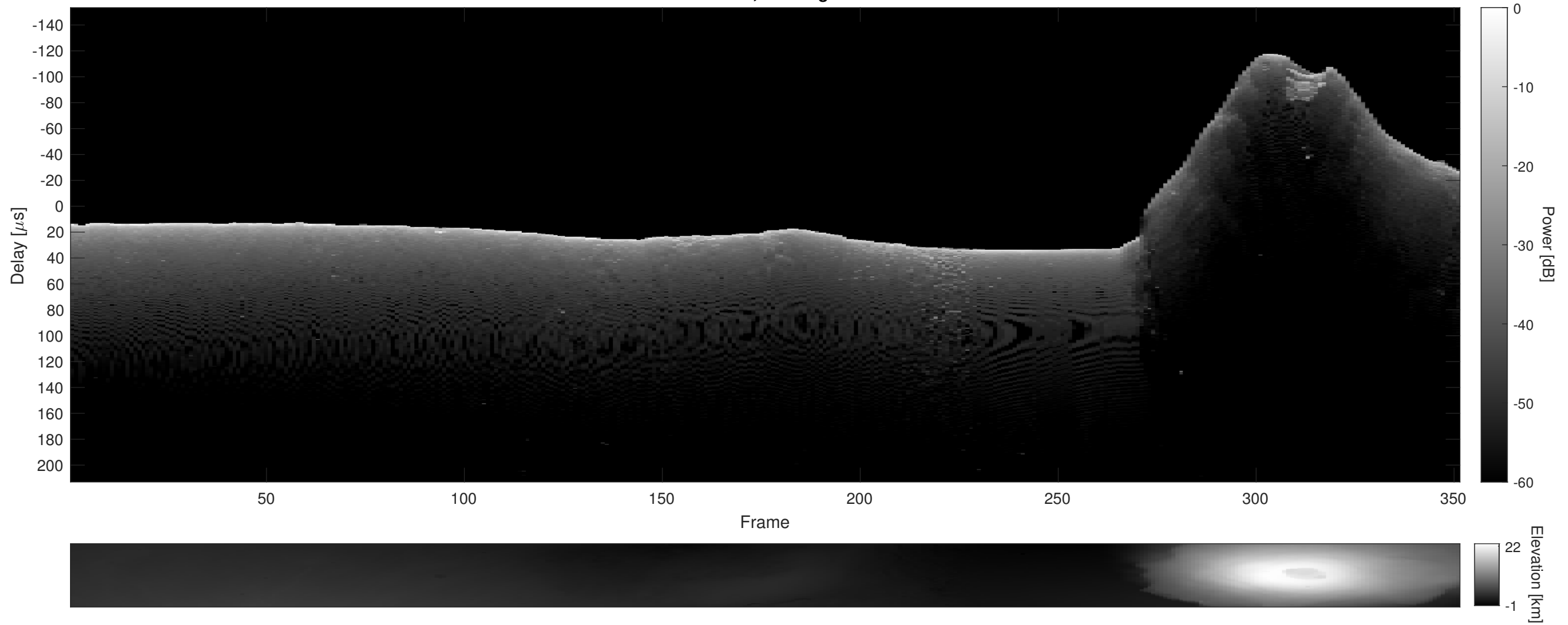
Orbit 8016, Cluttergram
