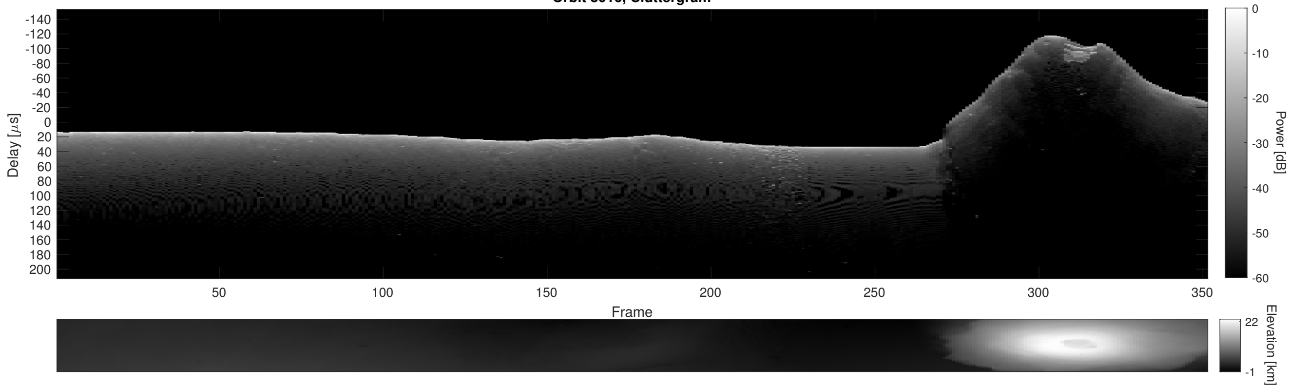
Orbit 8016, Cluttergram
