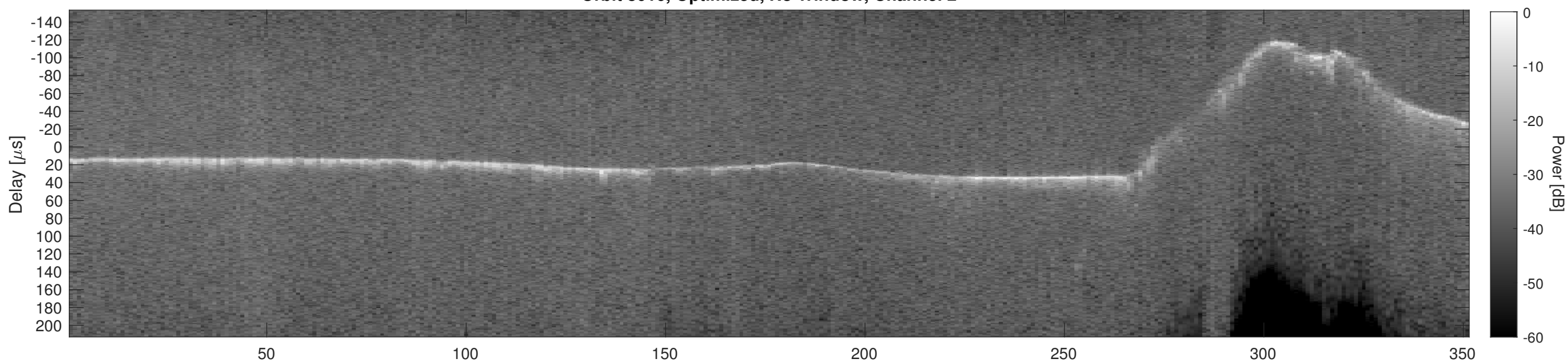
Orbit 8016, Cluttergram
