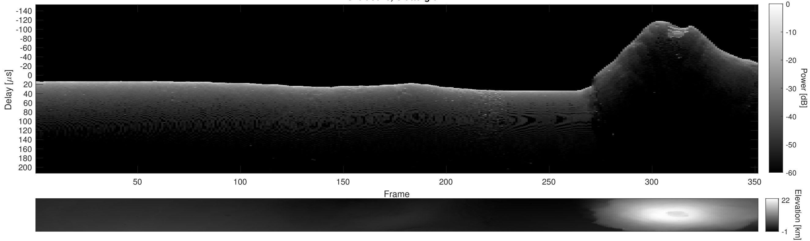
Orbit 8016, Cluttergram
