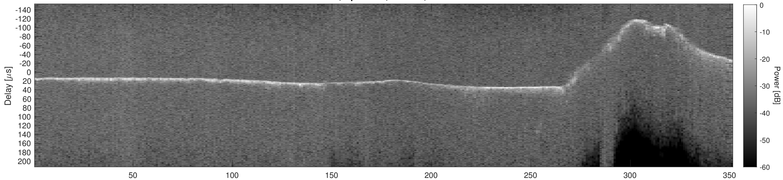
Orbit 8016, Cluttergram
