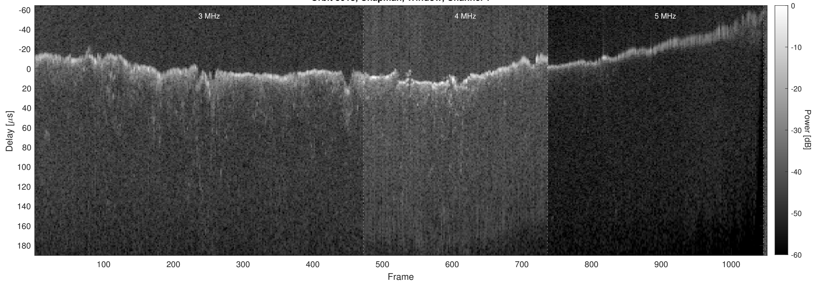
Orbit 8018, Chapman, Window, Channel 2
