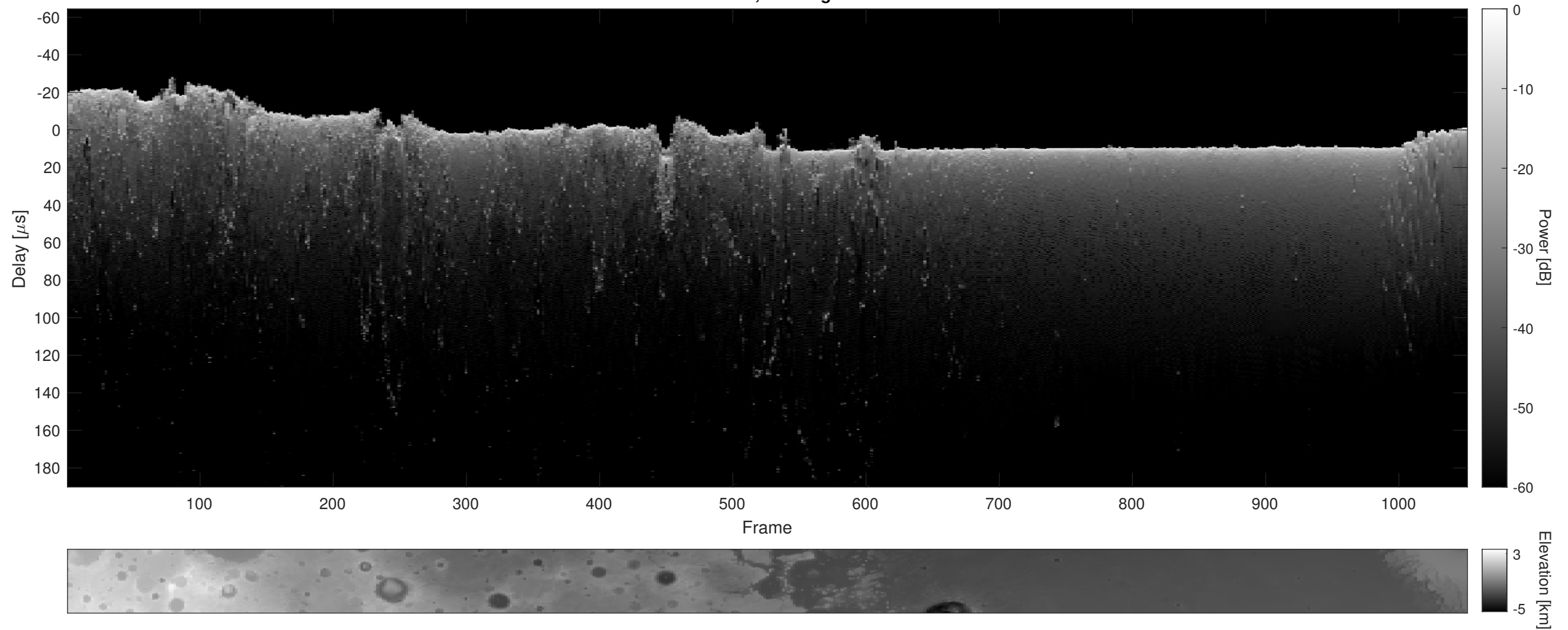
Orbit 8018, Cluttergram
