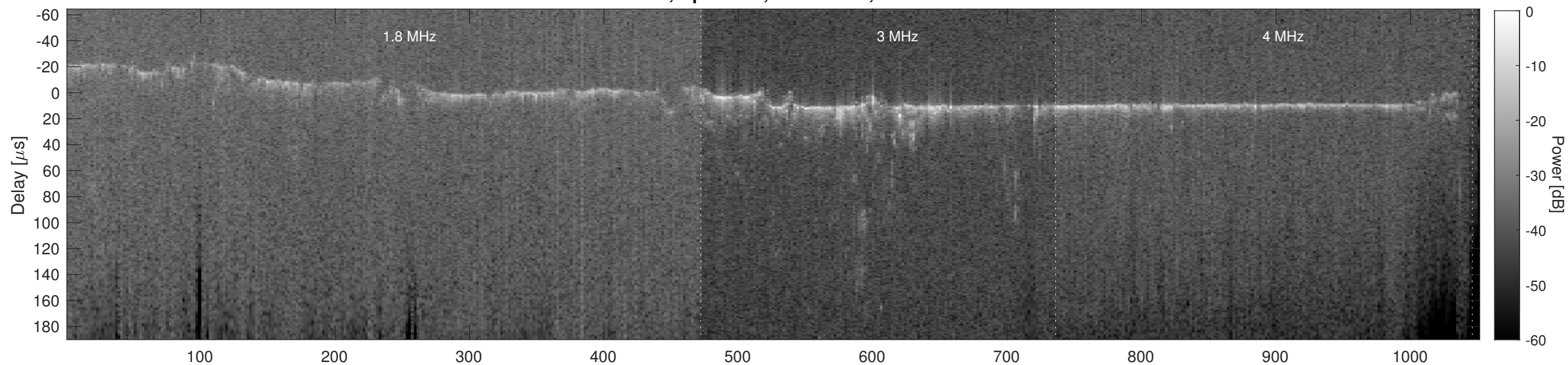
Orbit 8018, Cluttergram
