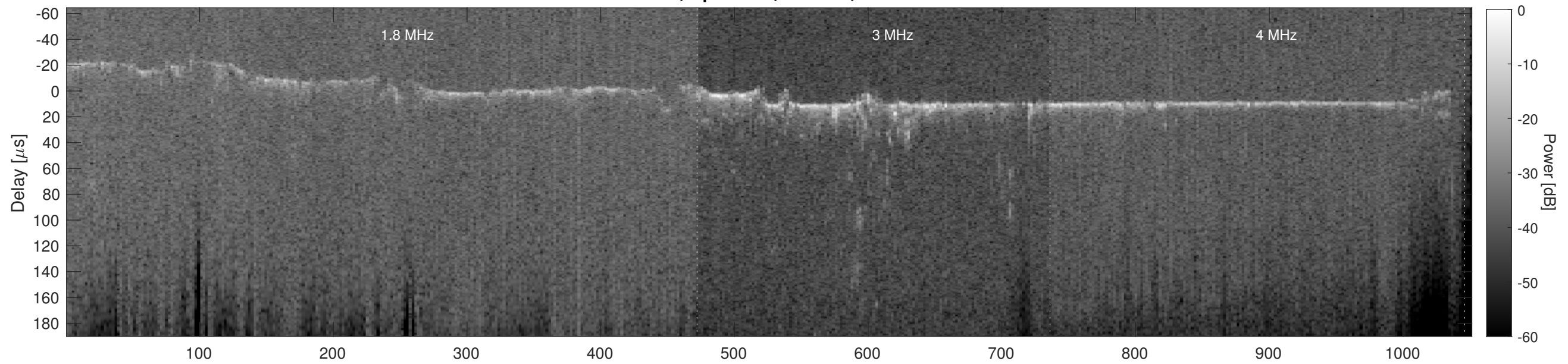
Orbit 8018, Cluttergram
