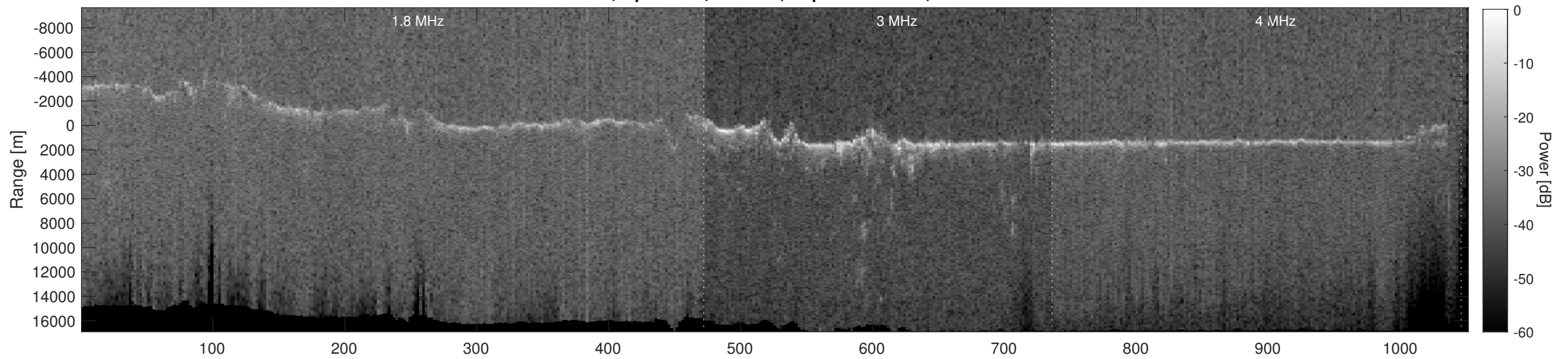
Orbit 8018, Depth-Corrected Cluttergram
