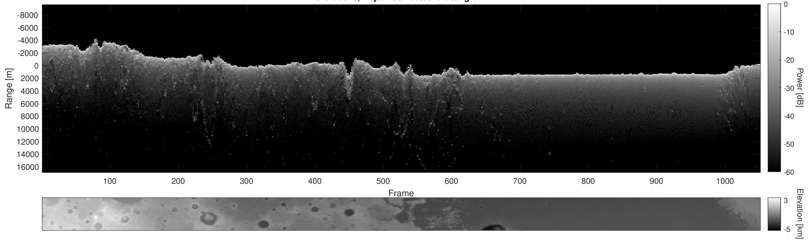
Orbit 8018, Depth-Corrected Cluttergram
