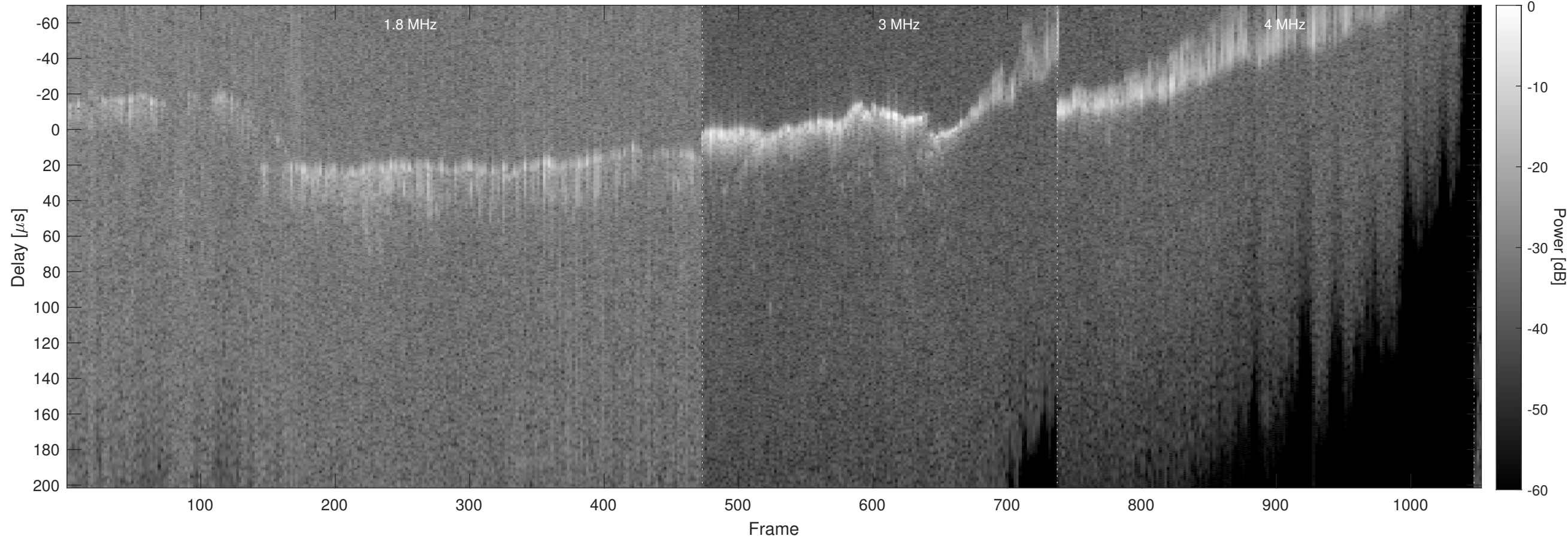
Orbit 8019, Chapman, No Window, Channel 2
