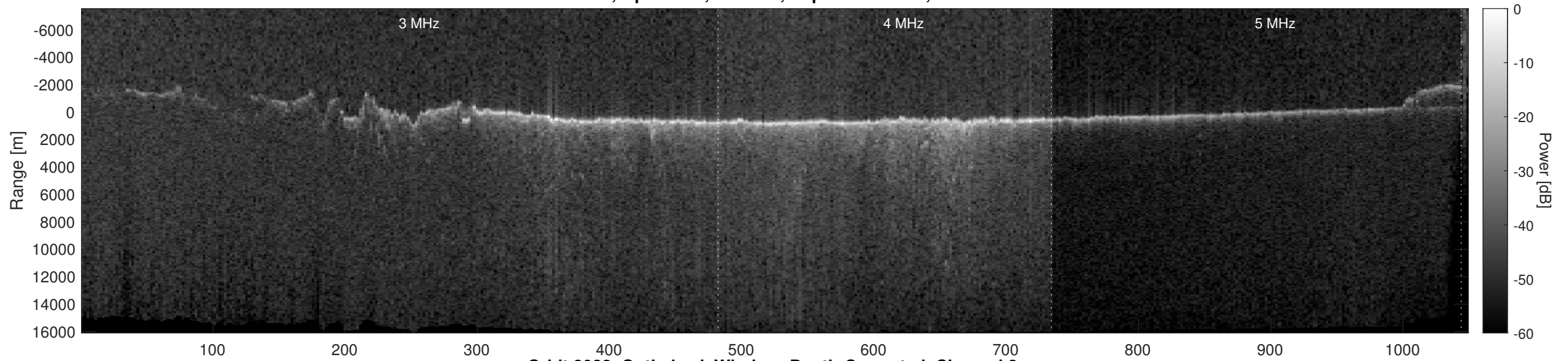
Orbit 8022, Optimized, Window, Depth-Corrected, Channel 2
