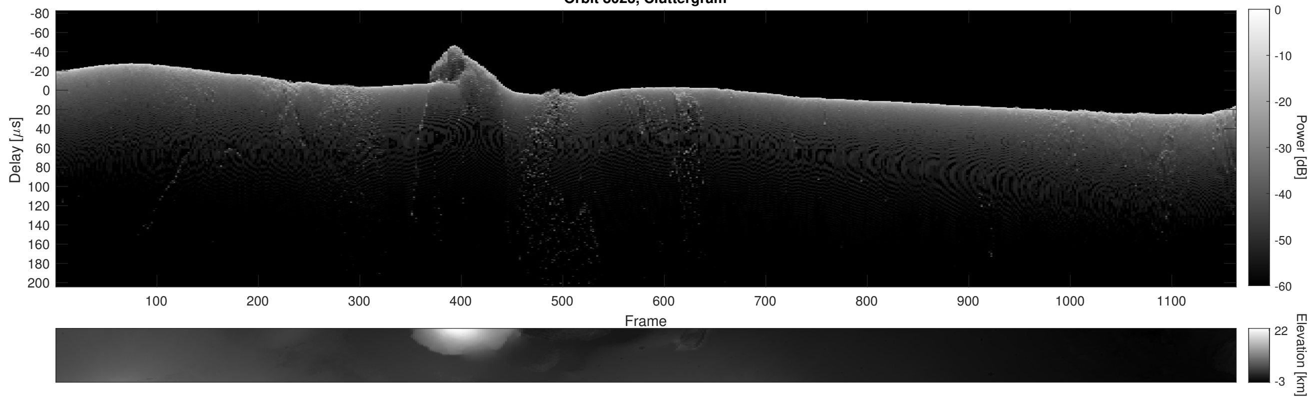
Orbit 8023, Cluttergram
