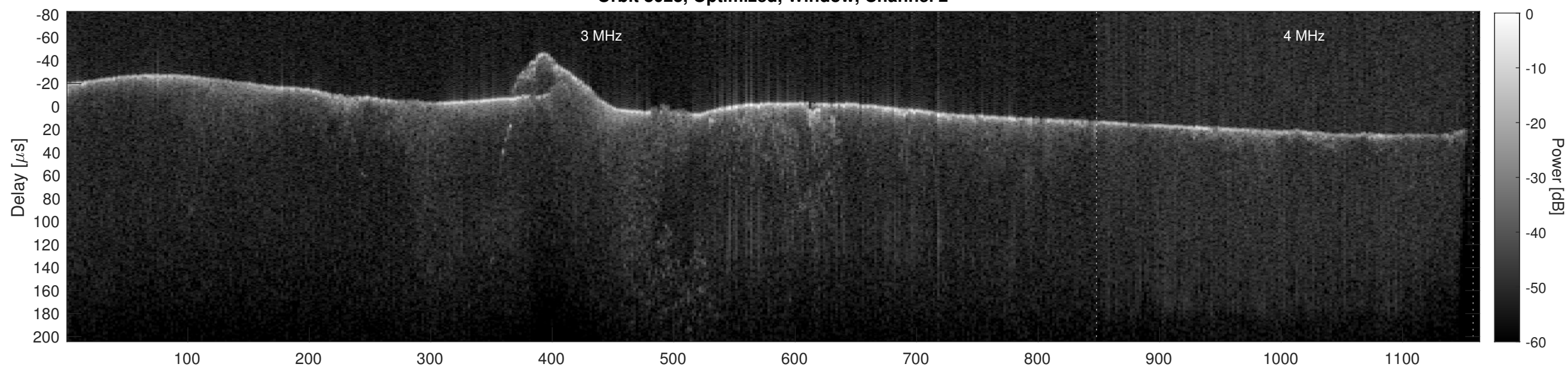
Orbit 8023, Cluttergram
