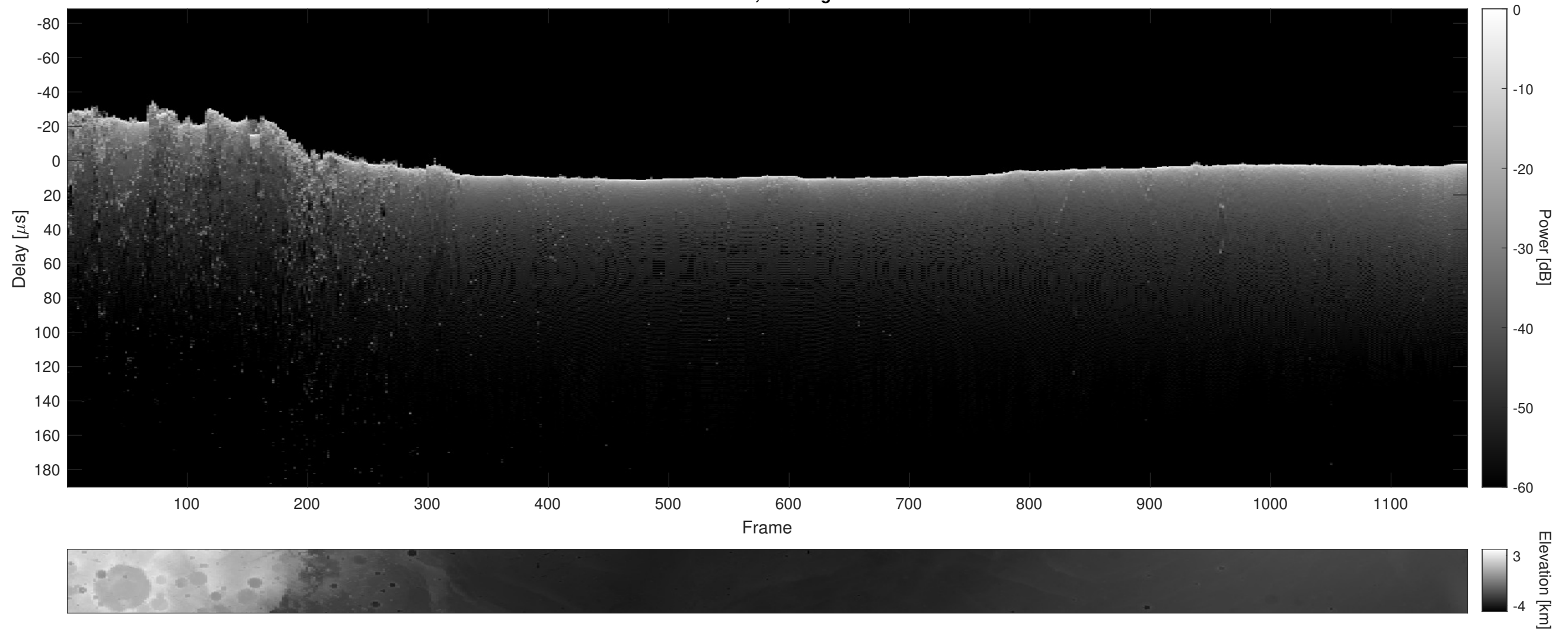
Orbit 8024, Cluttergram
