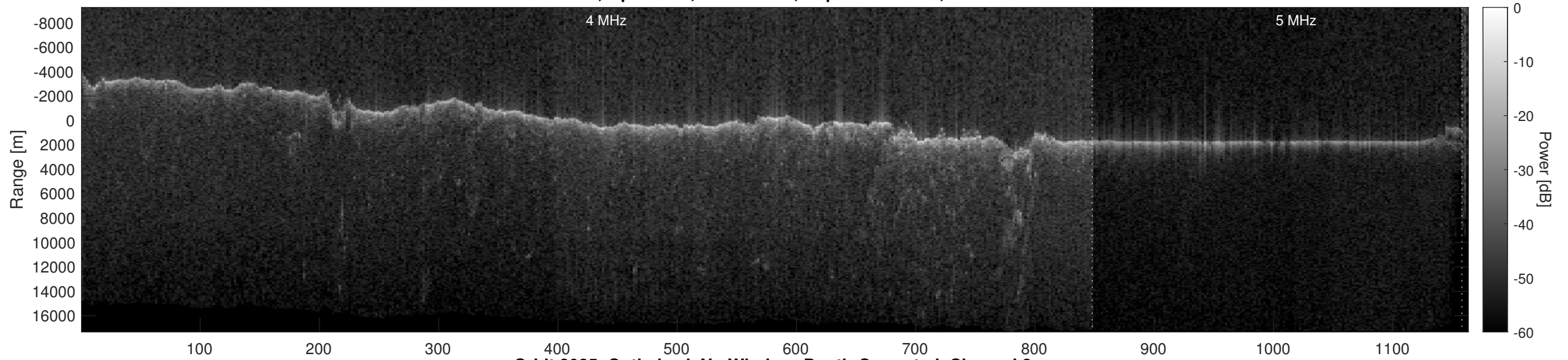
Orbit 8025, Optimized, No Window, Depth-Corrected, Channel 2
