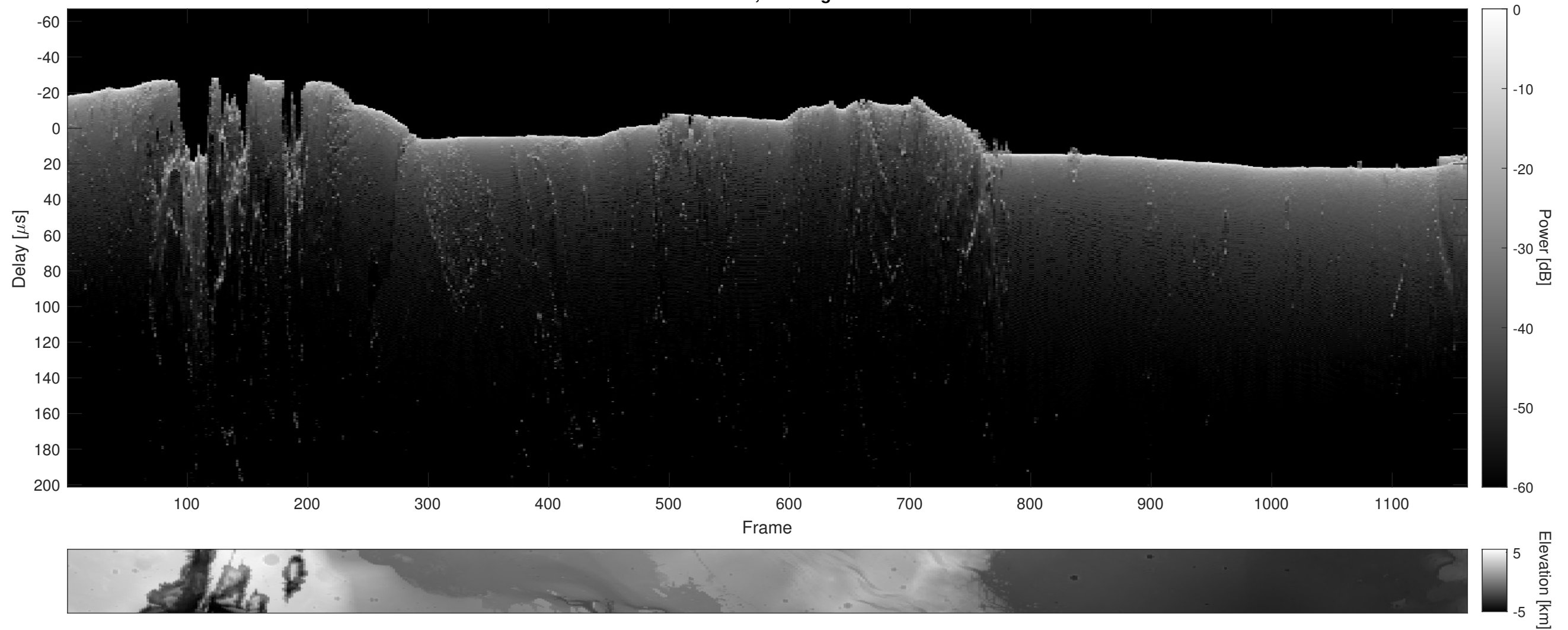
Orbit 8026, Cluttergram
