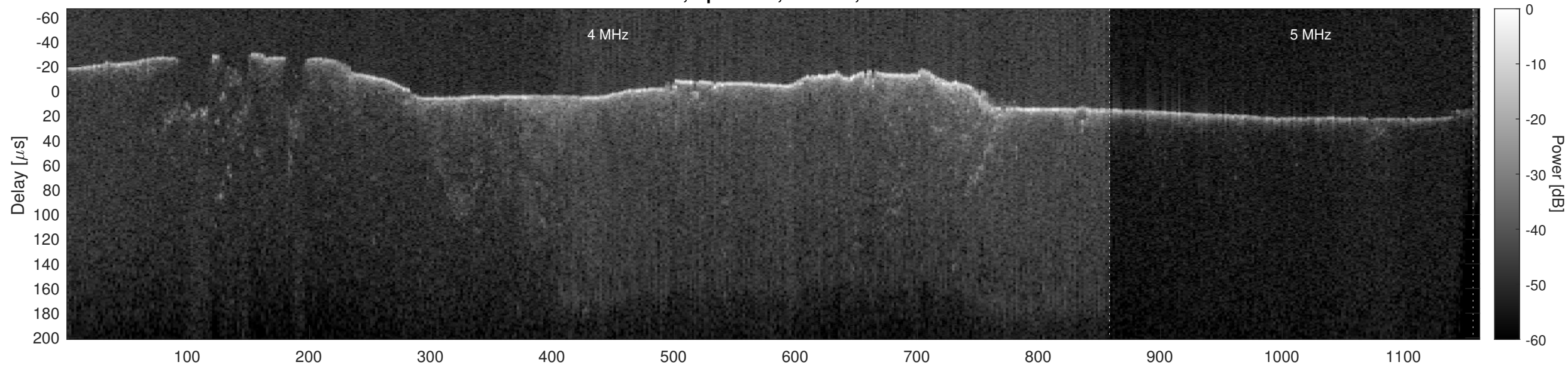
Orbit 8026, Optimized, Window, Channel 2
