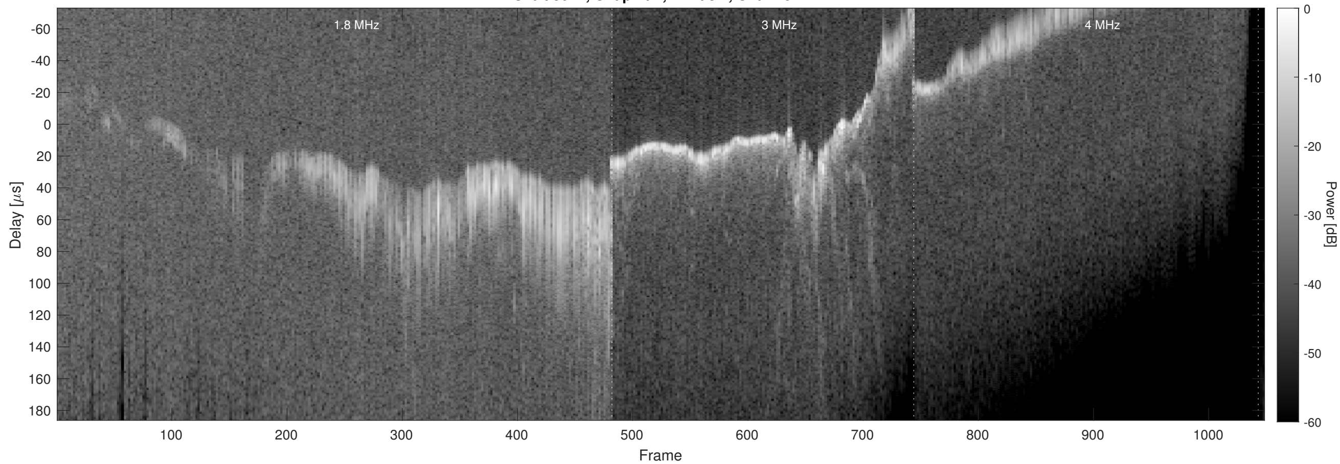
Orbit 8027, Chapman, Window, Channel 2
