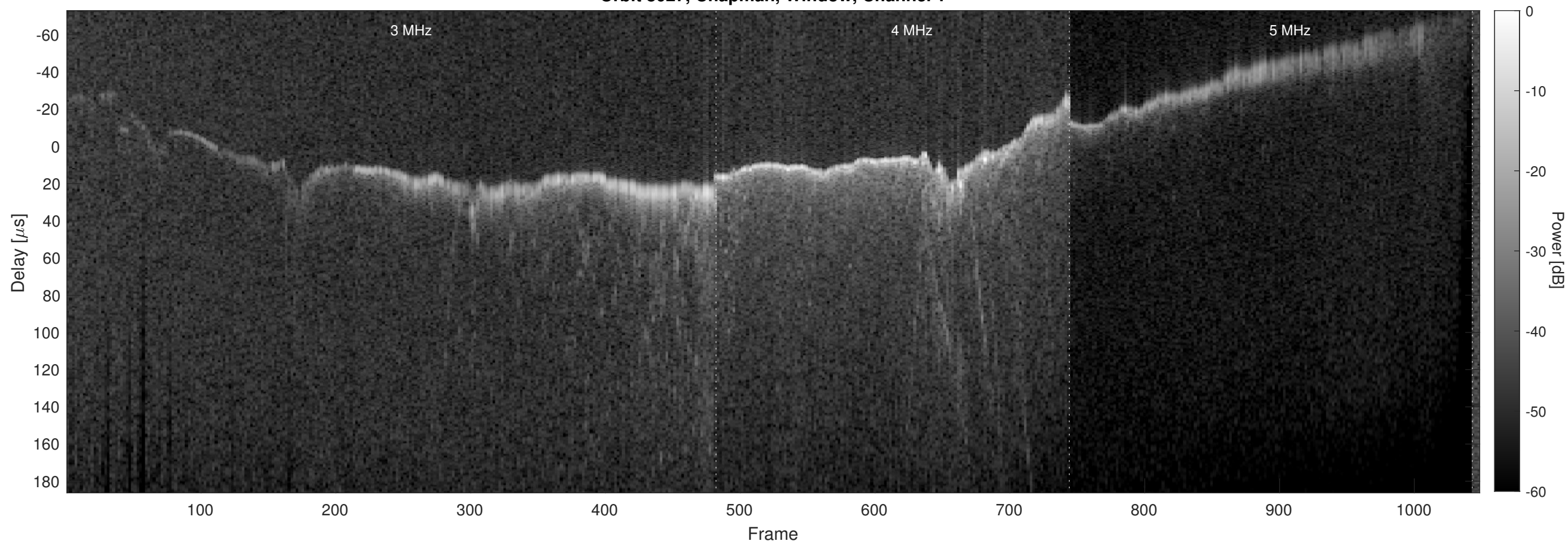
Orbit 8027, Chapman, Window, Channel 2
